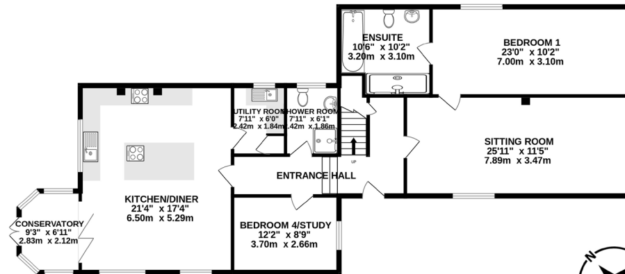
TOTAL FLOOR AREA : 2588 sq.ft. (240.5 sq.m.) approx.
