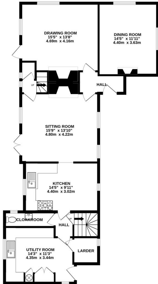
GROUND FLOOR 1053 sq.ft. (97.8 sq.m.) approx.
