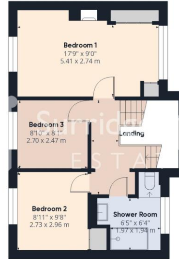
Floor 1
