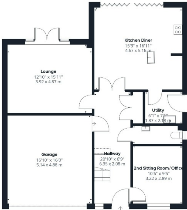
Floor 0
